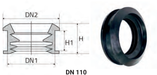
DN 110
