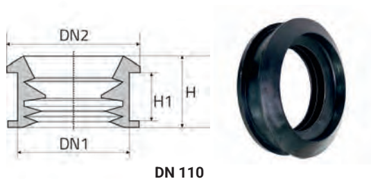
DN 110
